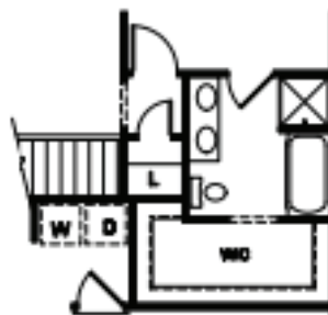
Alt. Primary Bath Layout
